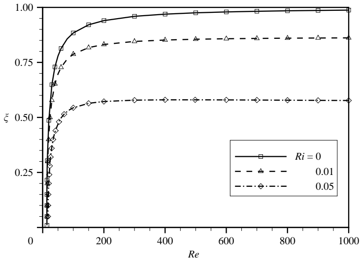
FIGURE 15. Neutral stability curves for the K-H temporal and spatial instability. The mixing layer flow is unstable below the curves and is stable above them. Pr=9 , R=3 , \lambda=0.5 , \alpha_z=0 .
