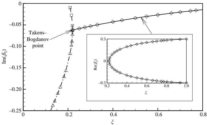
FIGURE 4. Dependence of the time amplification rate \text{Im}(\beta_1) on the depth of velocity layer \xi . Inviscid non-isothermal fluid flow, Ri = 0.2 , R = 3 , \lambda = 0.5 , \alpha_z = 0 . \Delta , first K-H mode; \square , second K-H mode; \diamond , Holmboe modes. The inset shows the dependence of \text{Re}(\beta_1) on \xi for the two Holmboe modes.
