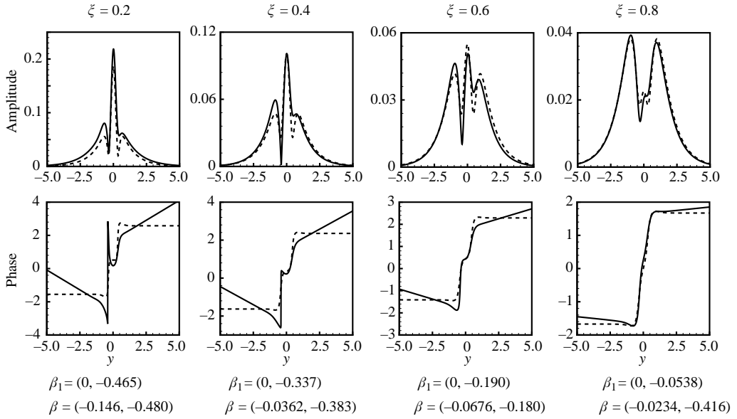
FIGURE 3. Amplitudes and phases of the temporal (dashed lines) and spatial (solid lines) perturbation of x -component of velocity for viscous isothermal mixing layer flow. \lambda = 1 , Re = 100 , \alpha_z = 0 .
