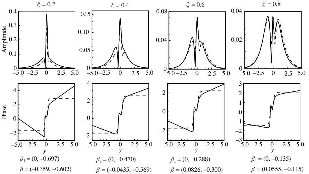
FIGURE 1. Amplitudes and phases of the temporal (dashed lines) and spatial (solid lines) perturbation of x -component of velocity for inviscid isothermal mixing layer flow. \lambda = 1 .
