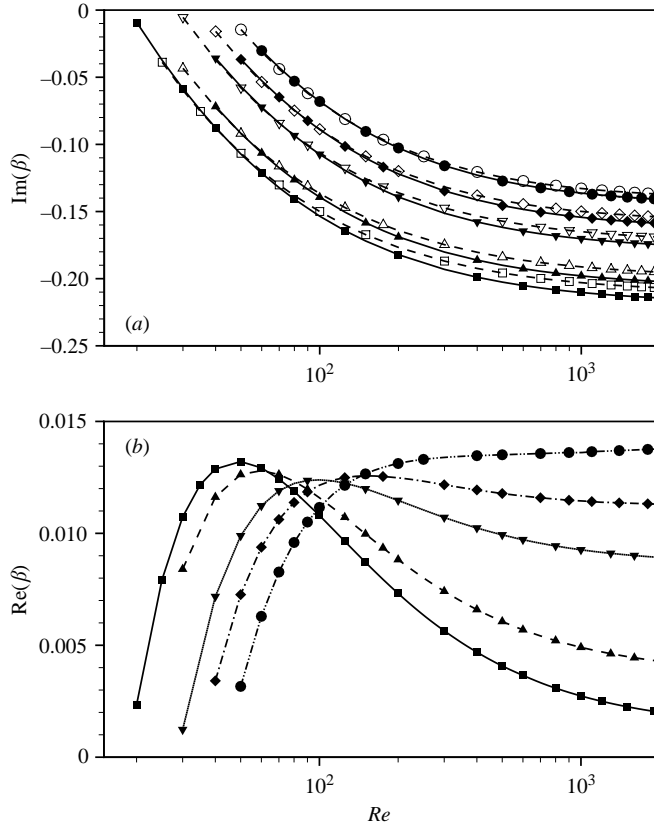
FIGURE 12. Dependence of parameter \beta on the Reynolds number for the temporal (open symbols) and spatial (filled symbols) K-H instability. Viscous non-isothermal flow, Pr = 9 , R = 3 , \lambda = 0.5 , \xi = 0.45 , \alpha_z = 0 . \square , \blacksquare , Ri = 0 ; \triangle , \blacktriangle , Ri = 0.01 ; \nabla , \blacktriangledown , Ri = 0.03 ; \diamond , \blacklozenge , Ri = 0.04 ; \circ , \bullet , Ri = 0.05 .
